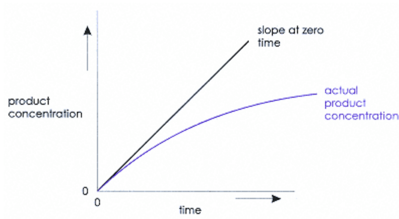
Figure 7.6. Time course for enzyme reaction. The purple line shows the product concentration (y axis) as a function of time (x axis) for an enzyme reaction. The black line indicates the initial slope of the curve. This initial slope is the initial velocity of the reaction.
