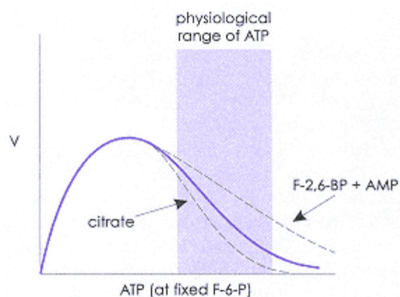
Figure 11.4. Effect of ATP on activity of phosphofructokinase. The effect of varying ATP at a fixed F-6-P concentration is shown as a solid line. The physiological range of ATP is shown in the shaded area. In the physiological range of ATP, increases in ATP concentrations are further inhibitory. In this range, citrate causes further inhibition of PFK and either F-2, 6-BP, or AMP causes some de-inhibition of the system, both shown with a dotted line.
