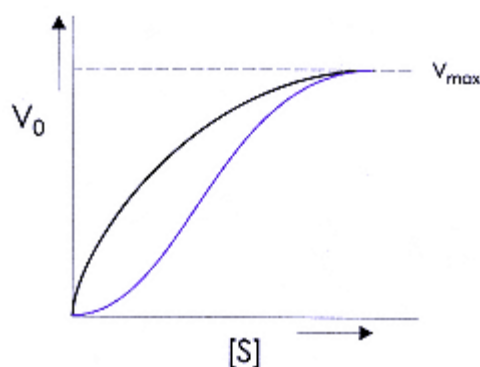
Figure 8.11. Sigmoid rate curve. The purple line shows how the reaction rate, for a reaction catalyzed by a cooperative enzyme, varies with the substrate concentration. For comparison, the black line shows the shape of the hyperbolic curve seen with reactions catalyzed by enzymes that obey the Michaelis-Menten equation.
