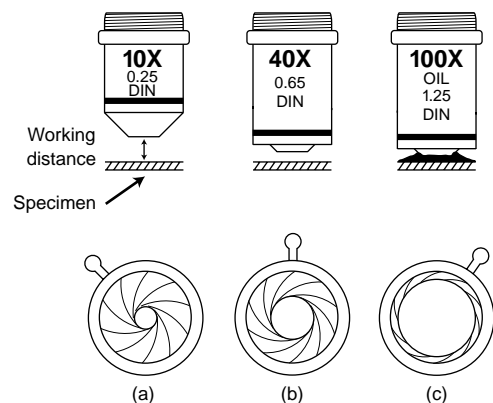
Fig. 4.3 Working distances of 10 \times , 40 \times , and 100 \times objectives and adjustment of condenser iris for each objective. (a) Iris about two thirds closed for 10 \times objective. (b) Iris open more for 40 \times objective. (c) Iris fully open for 100 \times objective. Note how closely the 40 \times and 100 \times objectives work to the slide.
