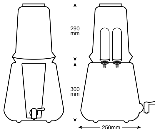
Fig. 4.8 Berkefeld polypropylene gravity water filter. Left: Front view. Right: Interior side view showing Sterasyl ceramic candle filters fitted.
