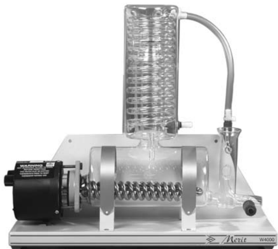
Plate 4.3 Merit water still. Courtesy of Bibby Sterilin.
