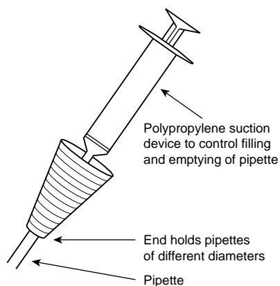
Fig. 4.17 Low cost controlled pipette filler that can be used with pipettes of different diameters.
