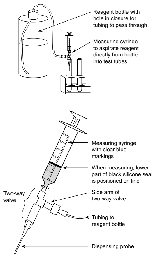
Fig. 4.19 DHT inexpensive manual syringe dispensing system. Upper : Complete system with reagent bottle, tubing and syringe (2.5 ml or 5.0 ml) with two-way valve. Lower : Measuring syringe with two-way valve suitable for measuring volumes up to 2.5 ml.
