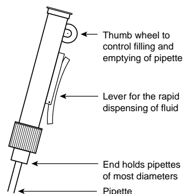
Fig. 4.18 Pi-pump 2500 for use with pipettes of 1 ml to 10 ml.
