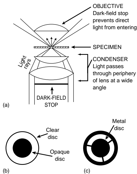
Fig. 4.4 (a) Principle of dark-field microscopy using a dark-field stop in the filter holder for the 10 \times and 40 \times objectives. (Courtesy Dr W G Hartley). (b) Dark-field stop made in the laboratory. (c) Manufactured metal dark-field stop.
