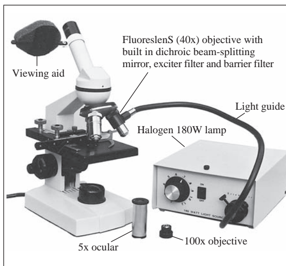
Incident fluorescence FluoreslenS system. Courtesy of Portable Medical Laboratories.
