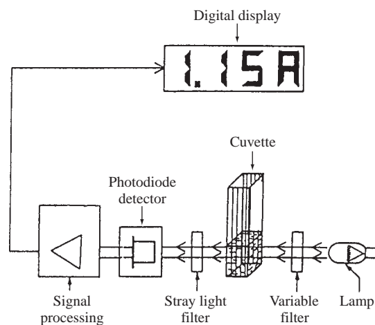
Fig. 4.20 Optical path of C0 7000 colorimeter.
