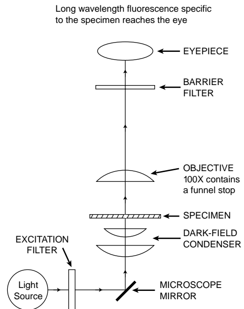
Fig. 4.5 Principle of transmitted light fluorescence.
