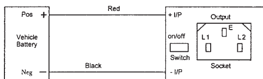
Plate 4.1 SM 2716 Switched Mode 200 Watt Handy Mains Inverter showing cable and clips for attachment to a 12 V lead-acid battery.
