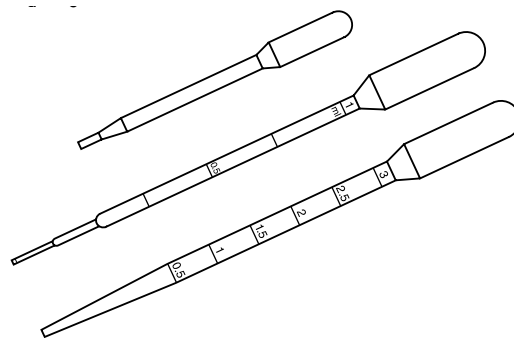
Fig. 4.16 Examples of useful graduated and non-graduated plastic (polyethylene) bulb pipettes ( Pastettes ).
