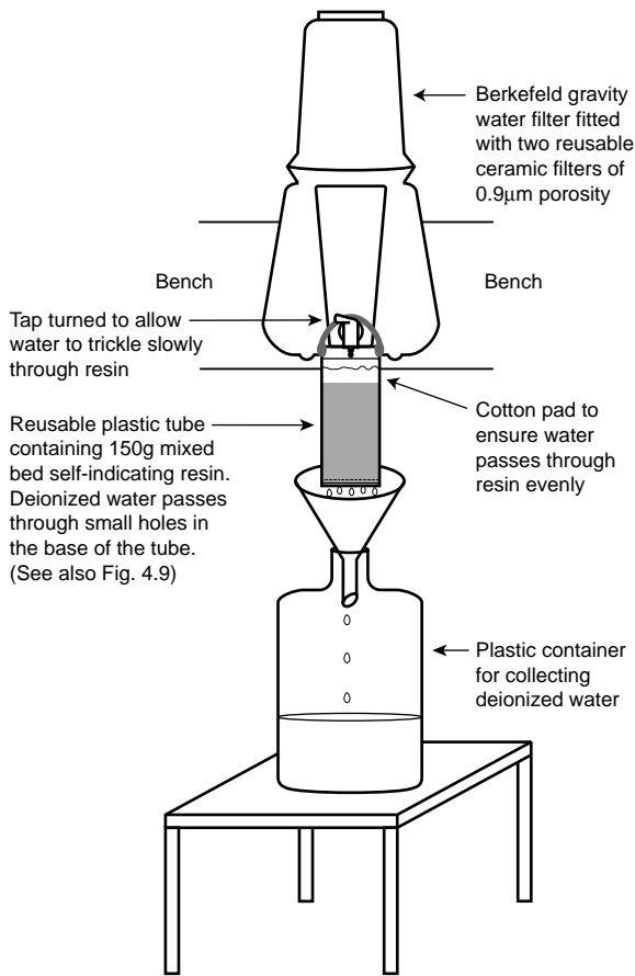
Fig. 4.10 Low cost practical method of obtaining pure water in district laboratories. The water is first filtered and then deionized using a laboratory-made deionizer column.
