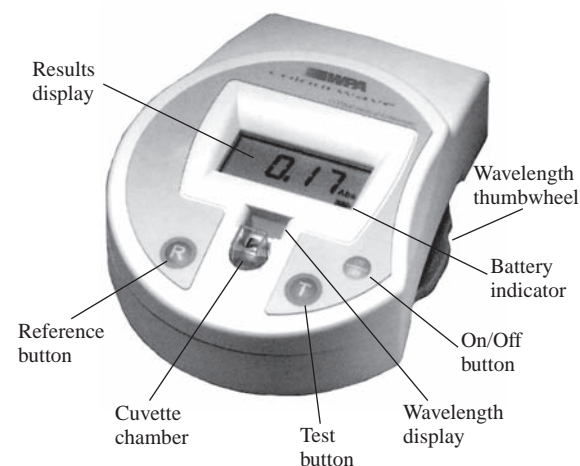
Plate 4.19 Controls of the Colourwave C0 7000 Colorimeter . Courtesy of Biochrom Ltd.
