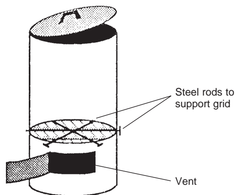
Fig. 3.6 Simple field incinerator Courtesy of the World Health Organization
