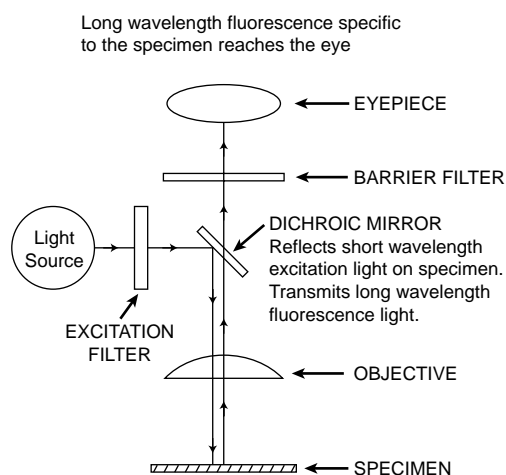
Fig. 4.6 Principle of incident (reflected) light fluorescence.
