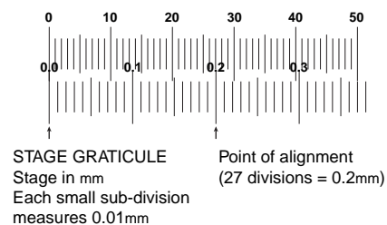
Fig. 4.7 Calibration of an eyepiece micrometer scale using a stage graticule scale calibrated in mm. Example shows 27 divisions of the eyepiece micrometer aligning with 0.2 mm (200 μm) of the stage graticule. One division is therefore equal to 200 divided by 27 = 7.4 μm.
