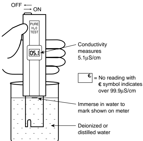
Fig. 4.11 Hanna Pure Water Test Meter.
