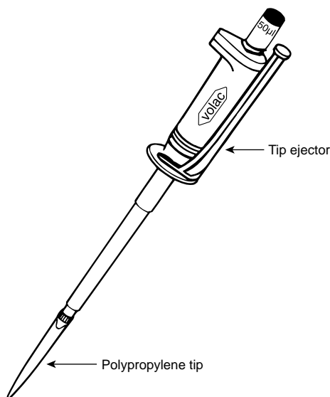
Fig. 4.14 Fixed volume Volac pipettor with built-in tip ejector.
