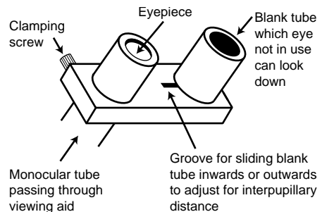
Fig. 4.2 Viewing aid for fitting to a monocular microscope (Elcomatic design).
