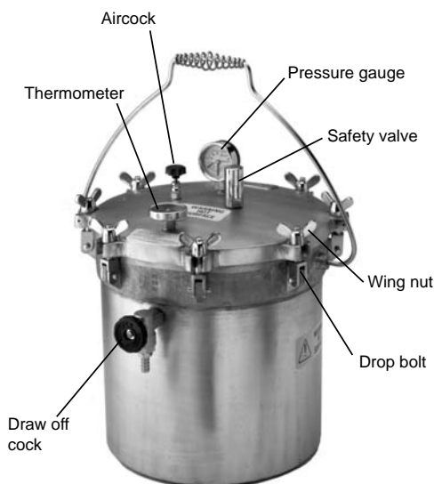
Plate 4.11 Dixon non-electric autoclave of 14 litre capacity, model ST 18, operating at 121 °C using an external heat source such as an electric hot plate, gas burner, or primus stove. Courtesy of Dixon Surgical Instruments.
