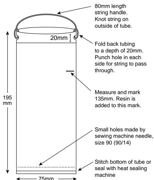
Fig. 4.9 Reusable polythene tube for holding deionizer resin.
