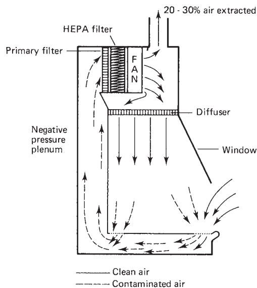
Fig. 3.4 Example of a Class II safety cabinet Reproduced from Laboratory Acquired Infections with permission of Butterworth and Co Publishers Ltd.
