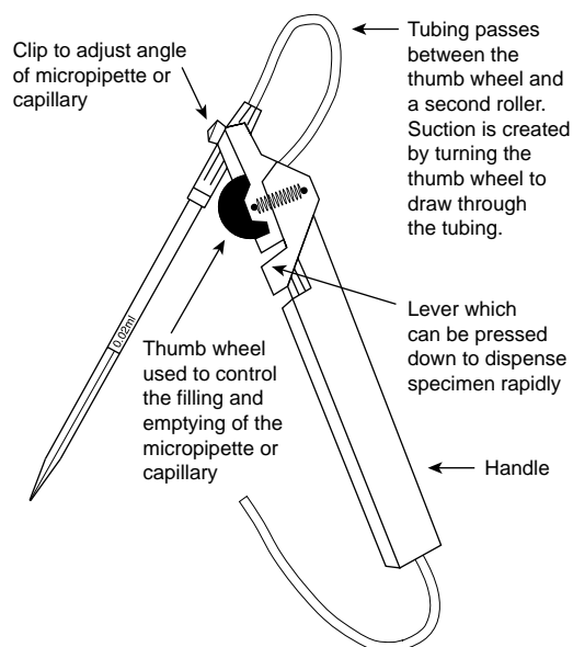
Fig. 4.13 Combined capillary and micropipette filler.
