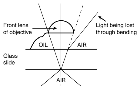
Fig. 4.1 Working principle of an oil immersion objective.
